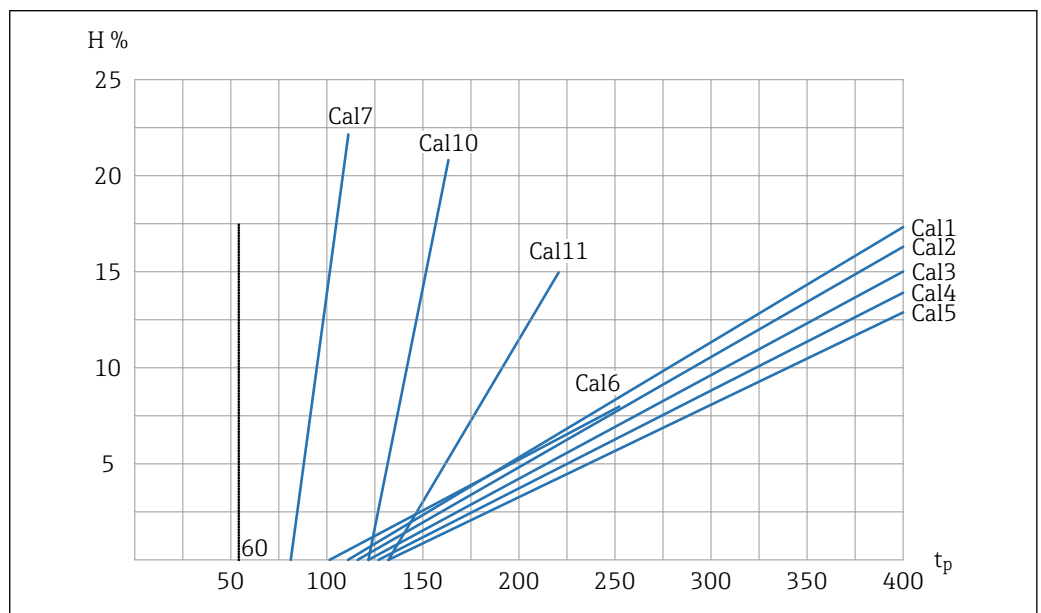
15 Lineaire kalibratiecurves (Cal1, Cal2, Cal3, Cal4, Cal5, Cal6, Cal7, Cal10, Cal11)
