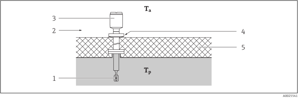
6 T_a Ambient temperature T_p Process temperature 1 Sensor 2 Temperature class, e.g. T6 3 Housing 4 Reference point: max. +85 °C 5 E.g. thermal insulation
