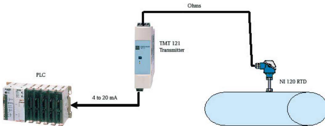
Monitoring system with TMT 121 transmitter
