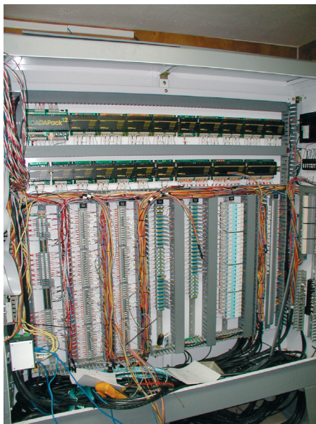
Control panel with TMT121 rail mounted transmitters
