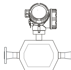
Proline Promass A 200 (type 8A2B or O8A2B)
