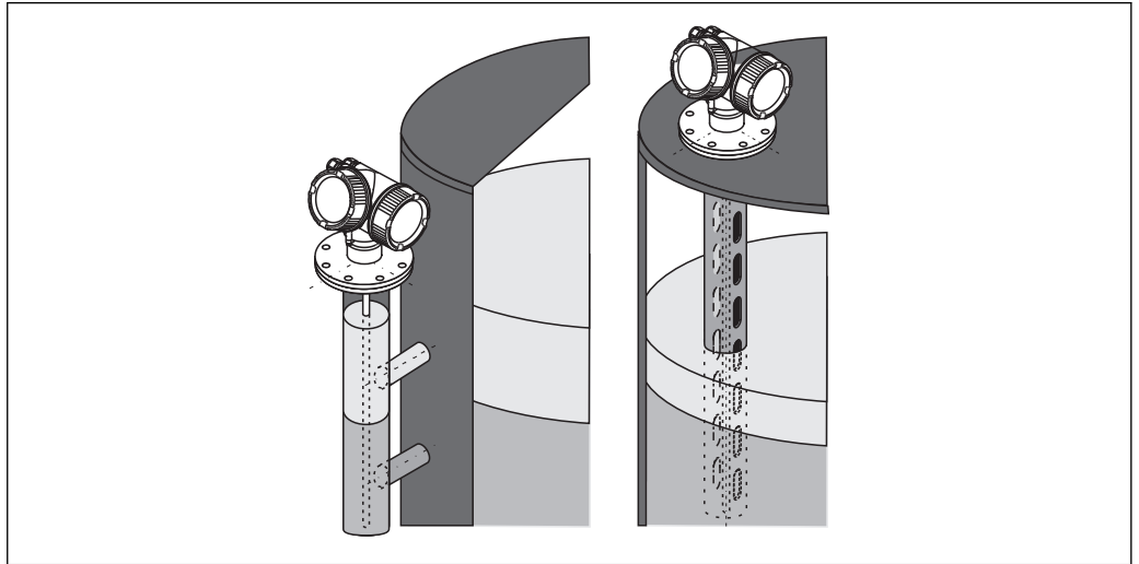
16 Mounting position of Levelflex FMP55
