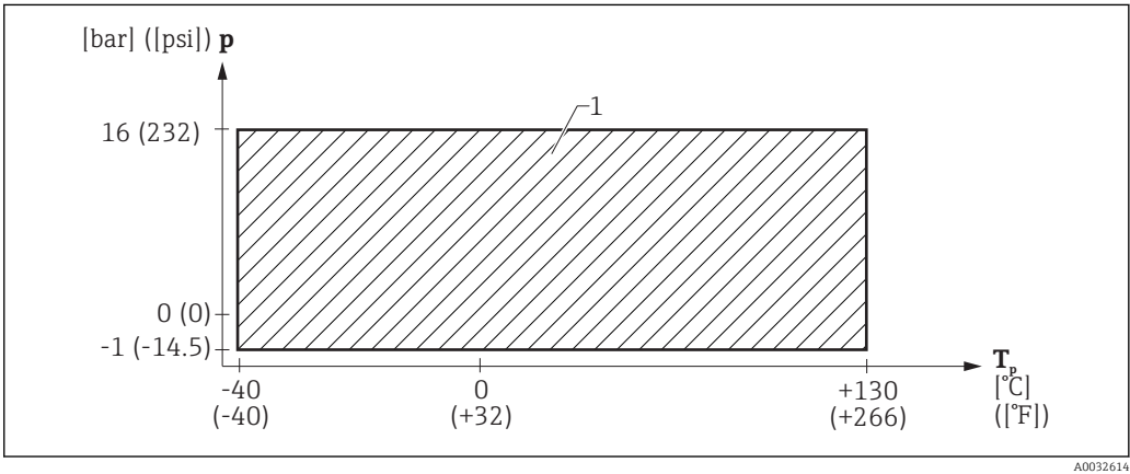
10 FMR60: Permitted range for process temperature and process pressure
