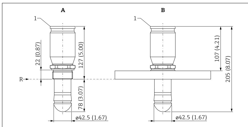
14 Dimensions: mm (in)
