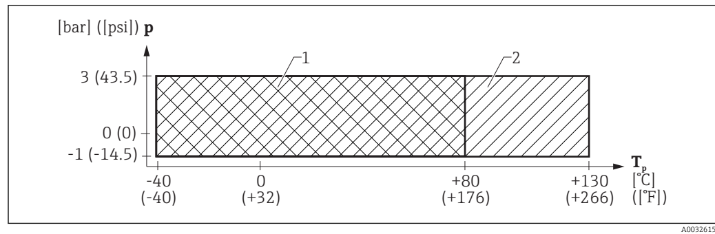
11 FMR60: Permitted range for process temperature and process pressure
