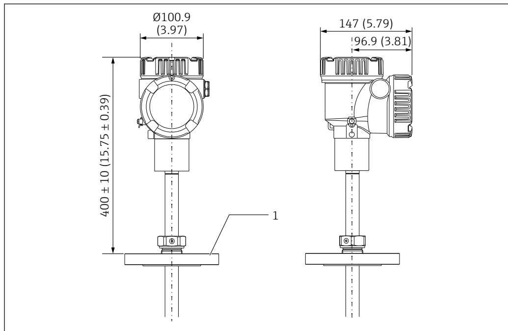
35 Adjustable flange. Unit of measurement mm (in)
