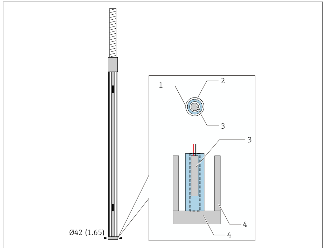
31 WB probe design. Unit of measurement mm (in)
