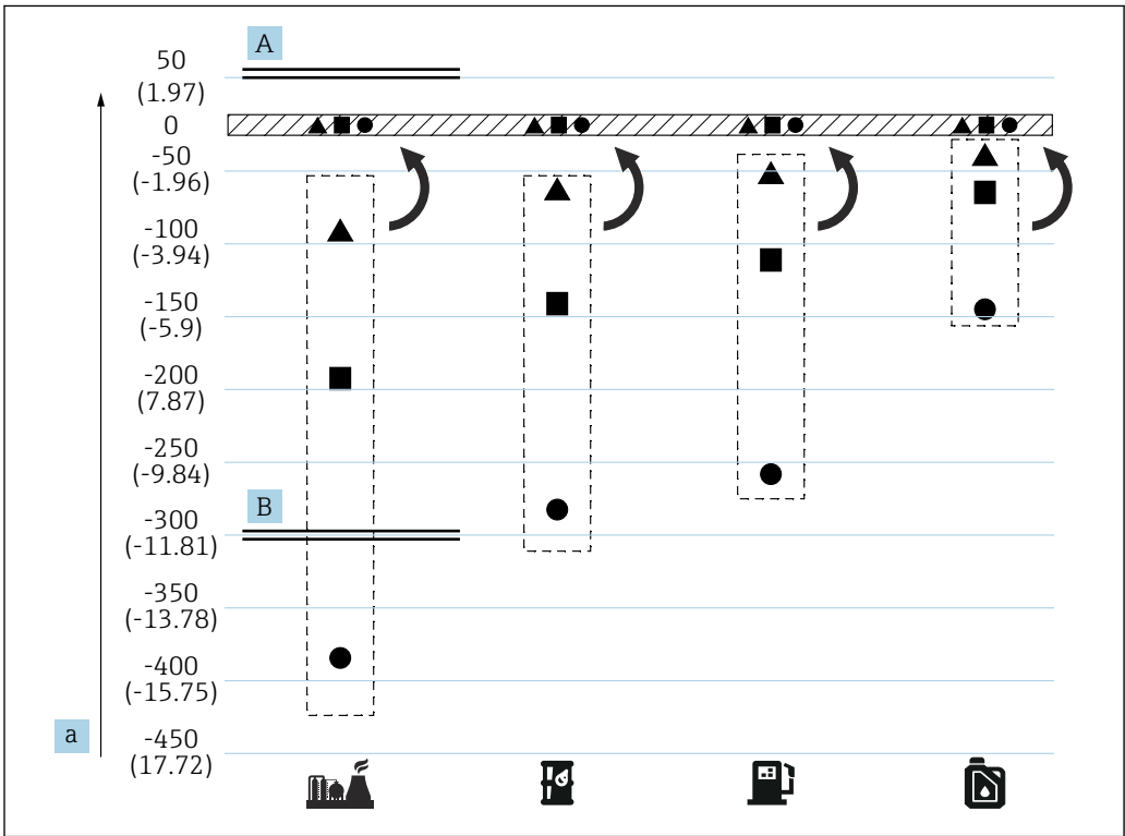
33 Effect of the three layers compensation
