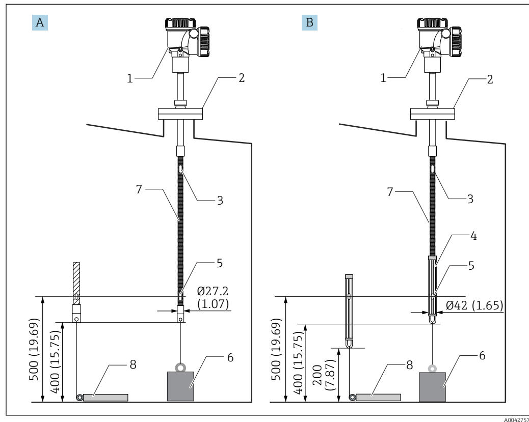
20 Anchor weight method. Unit of measurement mm (in)
