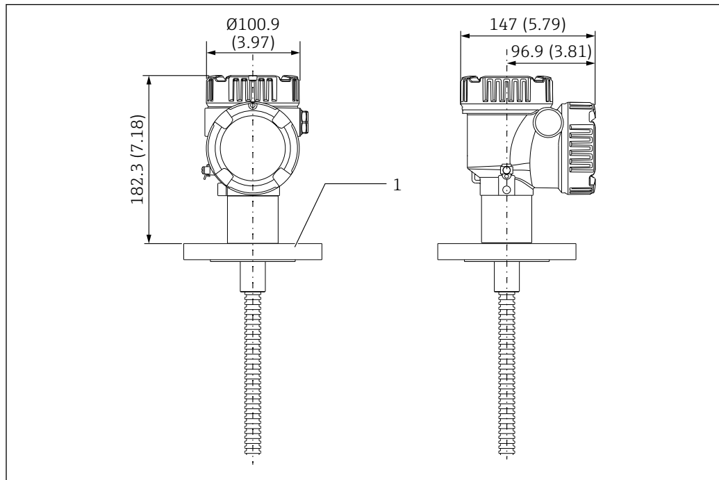
34 Welded flange. Unit of measurement mm (in)
