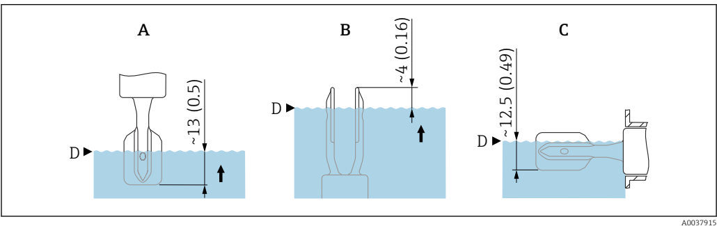
6 Switch point depending on the installation position. Unit of measurement mm (in) A Installation from above B Installation from below C Installation from the side
