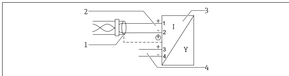
3 Blokdiagram PROFIBUS PA/FOUNDATION Fieldbus
