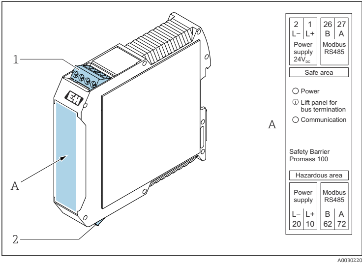
3 Safety Barrier Promass 100 with terminals
