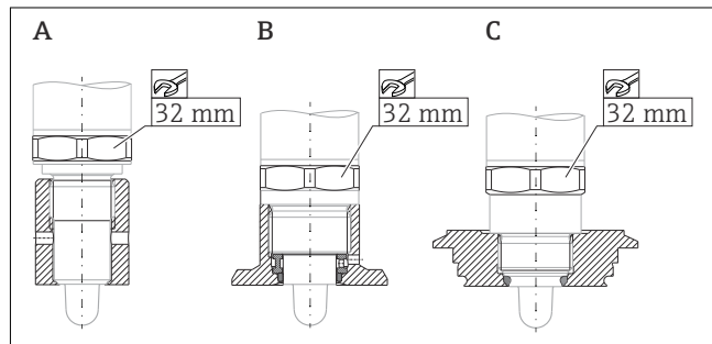
A Gwint G \frac{1}{2} " B Gwint G \frac{3}{4} " C Gwint M24 \times 1.5
