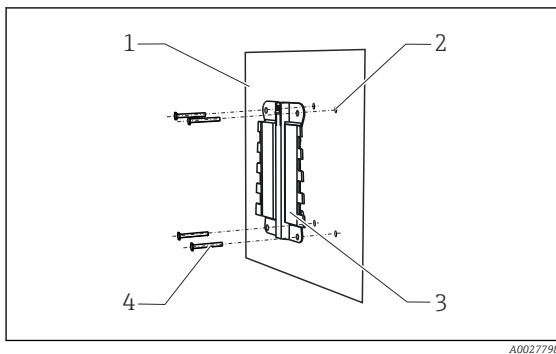
10 Wandmontage
