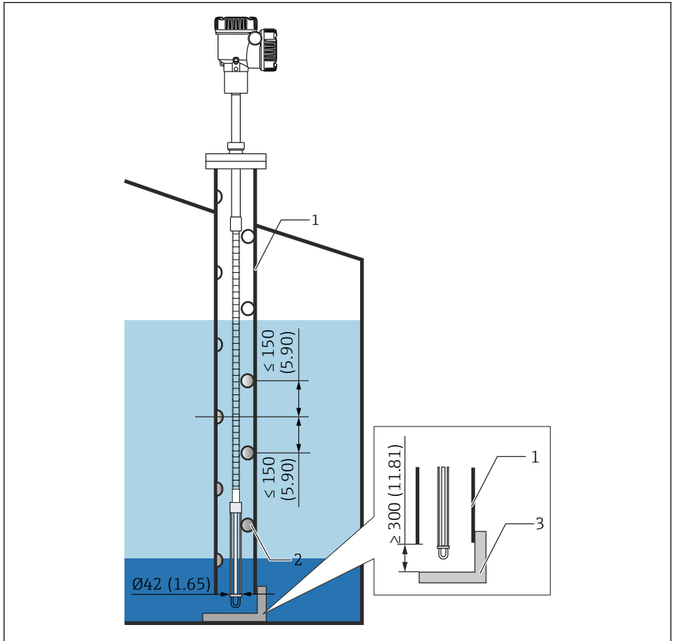
25 Stilling well. Maateenheid mm (in)
