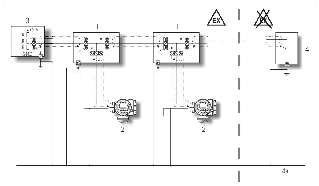
Fig. 10: Example for connecting potential equalization lines
