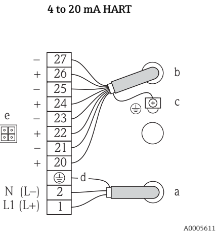
Fig. 12: Electrical connections
