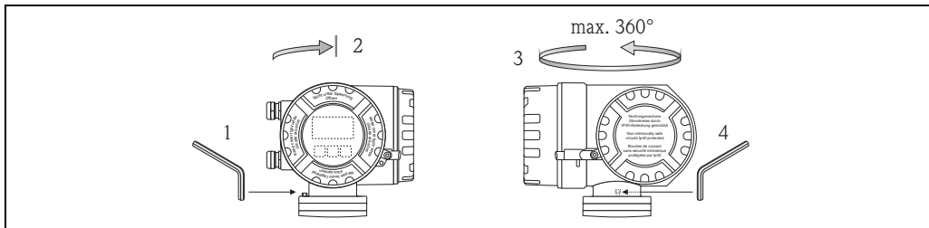
Fig. 7: Turning the transmitter housing
