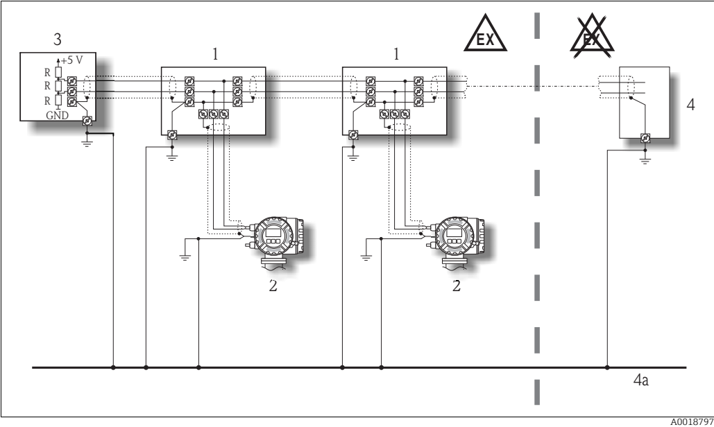
Abb. 5: Example for connecting potential equalization lines
