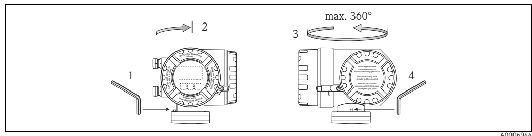
Abb. 4: Turning the transmitter housing
