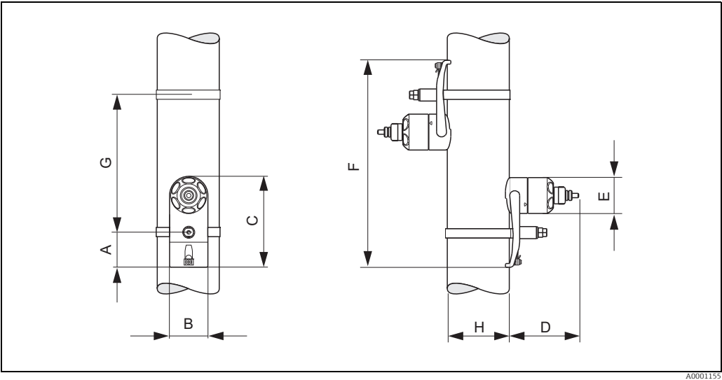
Mounting arrangement for measurement via one traverse
