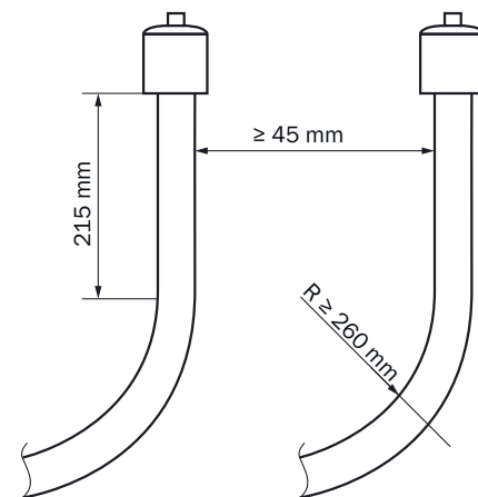
Figure 5: Lines – clearance and bending radius
