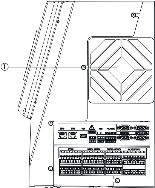
Figure 13: Electronic housing (right side)
