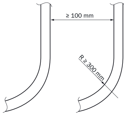
Figure 8: Lines – clearance and bending radius
