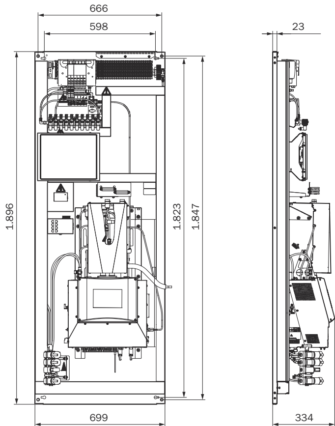
Figure 14: MCS200HW-MP (dimensions in mm)
