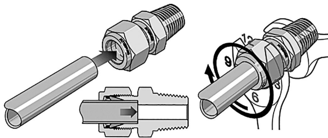
Figure 6: Stainless steel screw fitting
