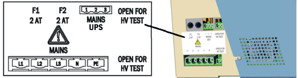
Figure 11: Voltage supply connections
