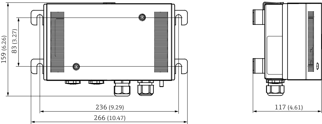
Sensor unit VISIC50SF closed (dimensions in mm (inch))
