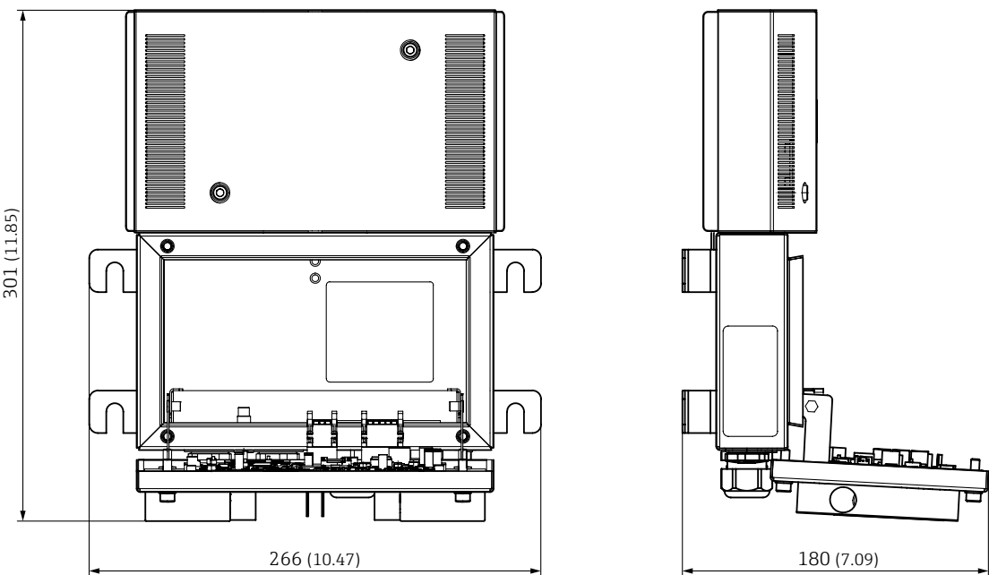
VISIC50SF sensor unit open with clipped-on front cover (dimensions in mm (inch))
