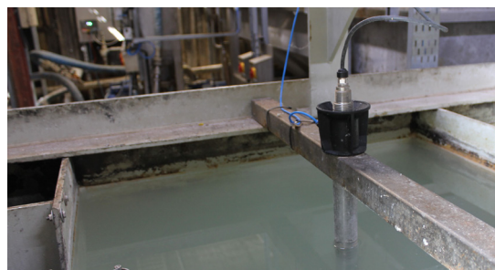
CAS80E sensor installed directly in the tank
