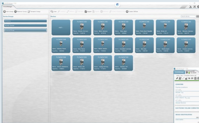
Device Manager
