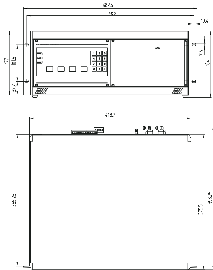
Fig. 43: 19" rack dimensions in mm
