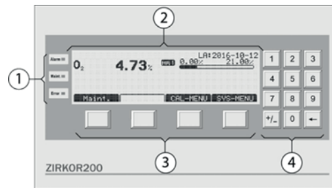
Fig. 25: Operating elements and display
