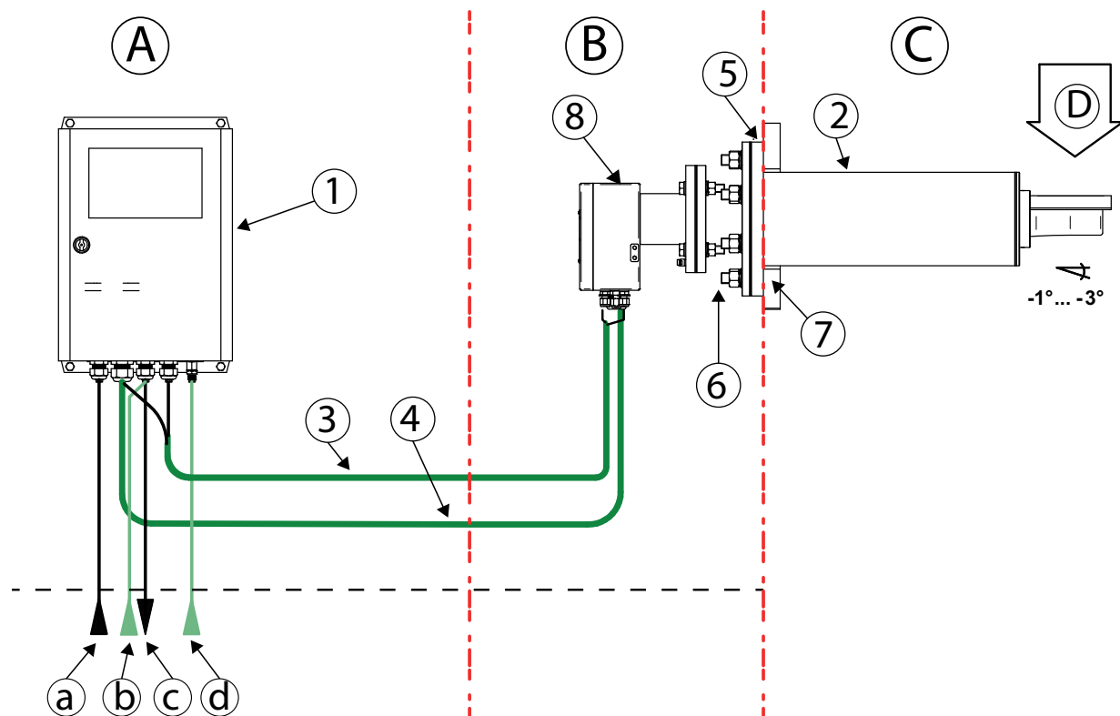
Fig. 5: System overview
