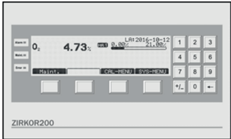
Fig. 53: Display board
