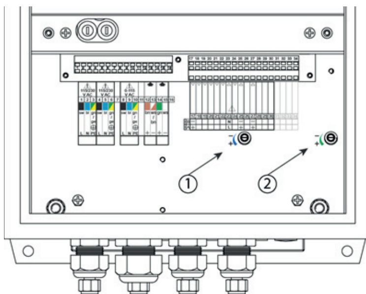
Fig. 33: Controller positions for reference air (1) and test air (2) (instrument air version)
