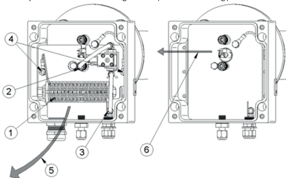
Fig. 38: Analyzer electronics when removing the inner part of the measuring probe
