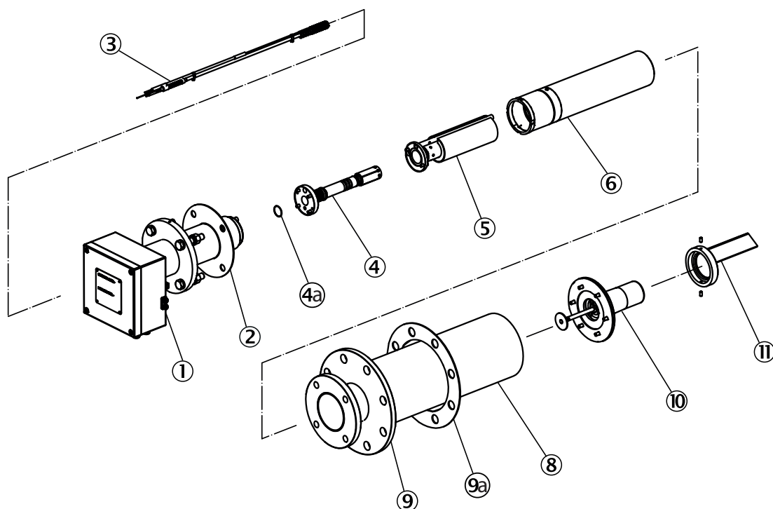
Fig. 48: Analyzer unit components
