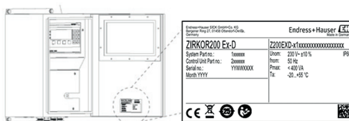
Fig. 2: Type plates (1)
