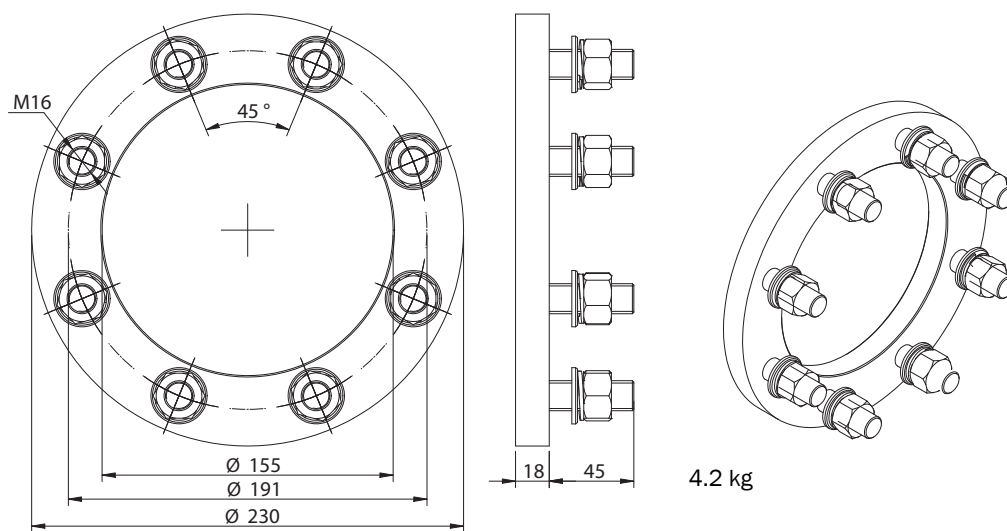
Fig. 46: Counter flange dimensions 5340177
