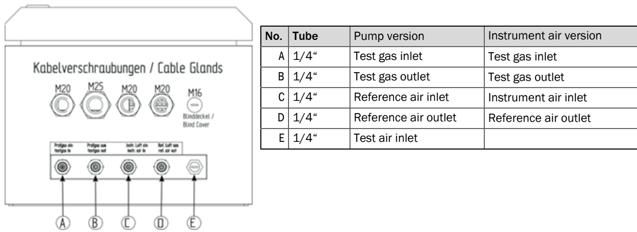
Fig. 21: Pneumatic connections, 19" rack, rear
