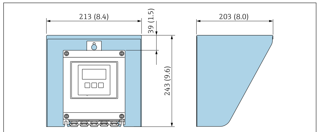
20 Protective cover for Proline 500 – digital; unit mm (in)
