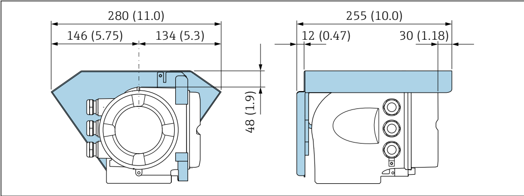
21 Protective cover for Proline 500; unit mm (in)
