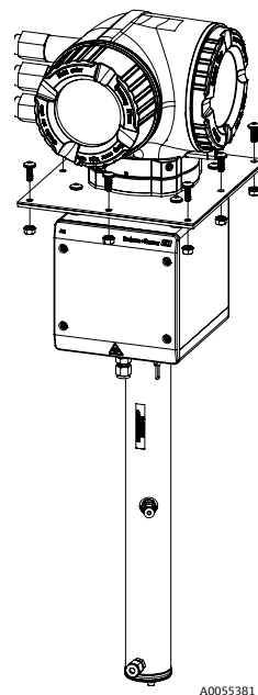
Figure 11. J22 plate mounting bracket and hardware
