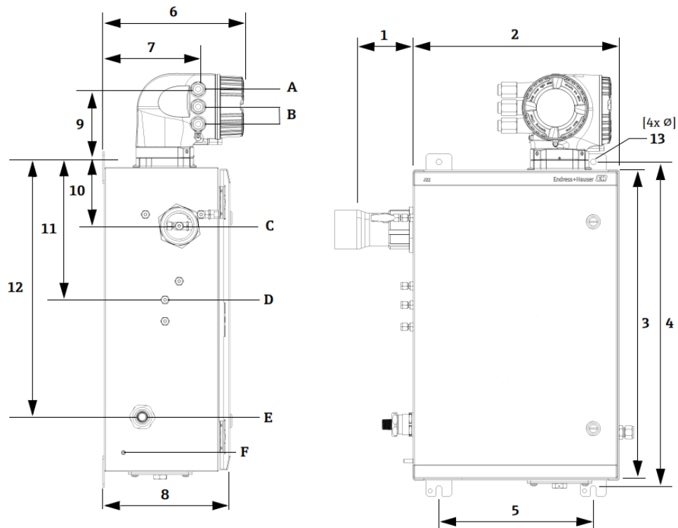
Figure 8. Mounting dimensions, J22 TDLAS Gas Analyzer with enclosed SCS
