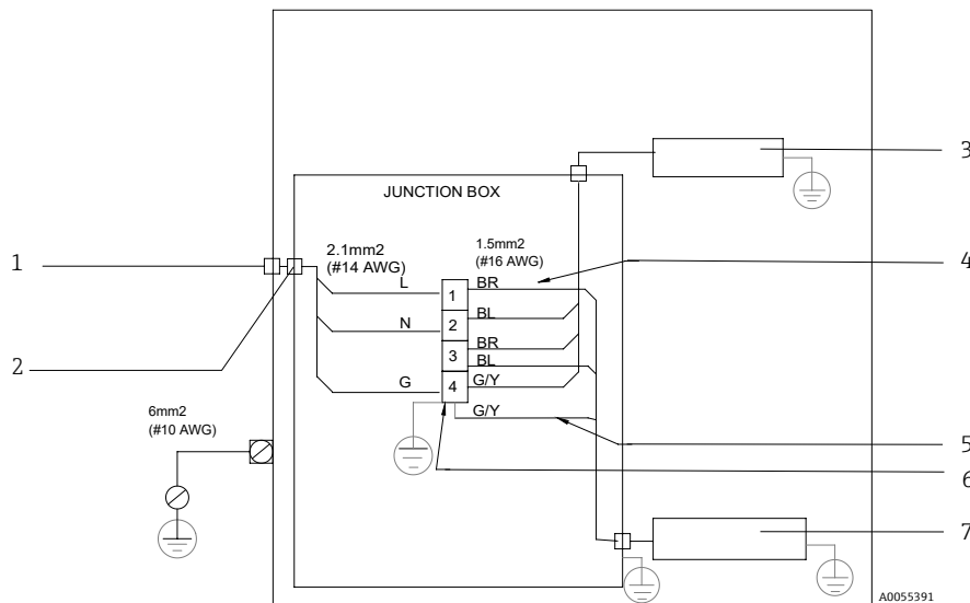
Figure 15. J22 SCS enclosure electrical connections
