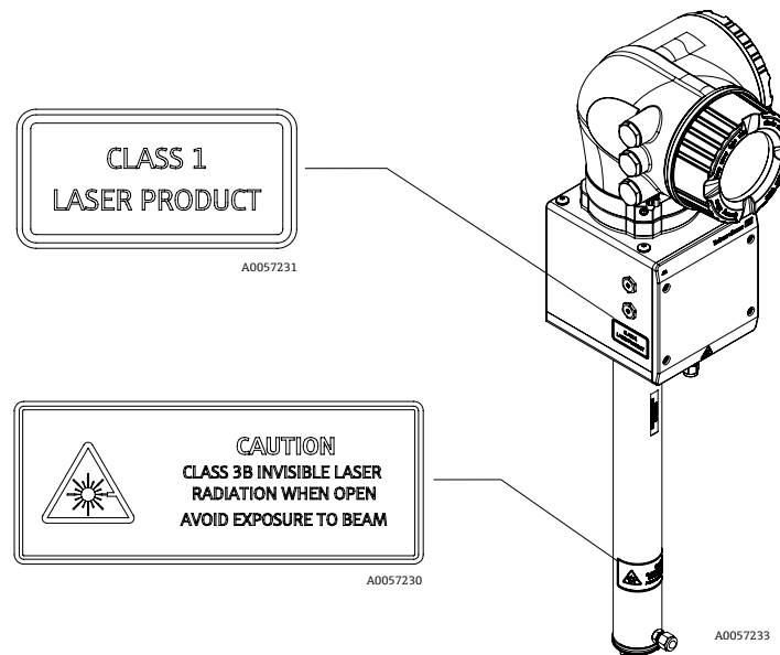
Figure 5. Location of laser safety labels
