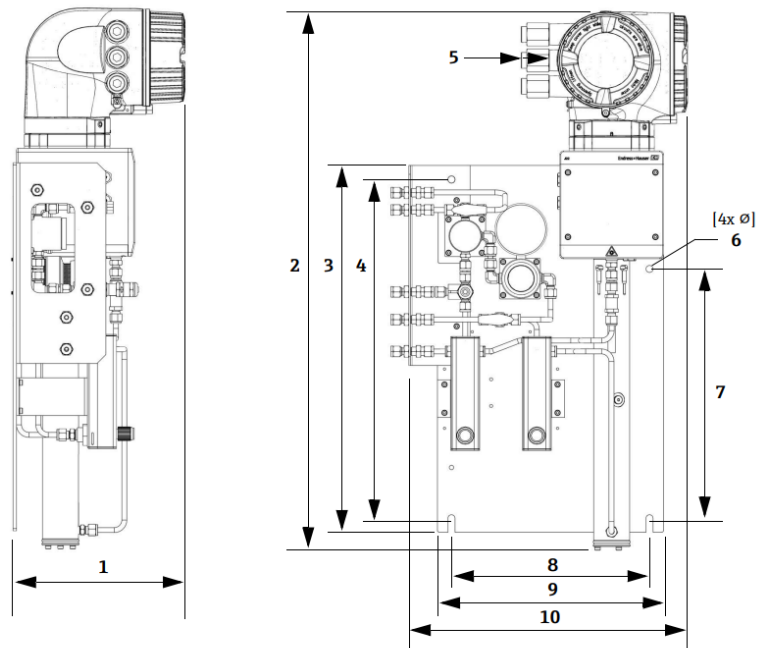
Figure 7. Mounting dimensions, J22 TDLAS Gas Analyzer with SCS on panel
