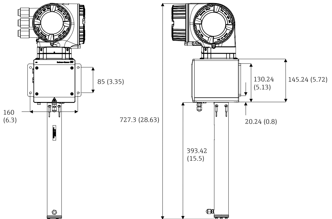
Figure 6. J22 TDLAS Gas Analyzer wall mount (without panel) mounting dimensions, mm (in)
