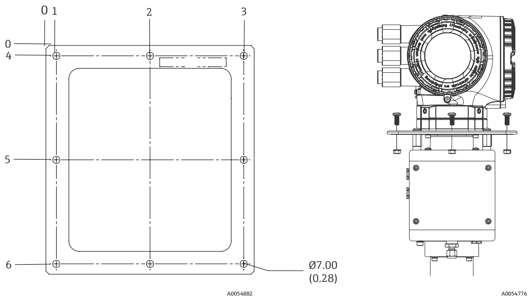
Figure 13. Enclosure mounting plate and hardware. Engineering units: mm (in)
