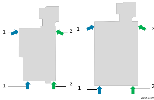
Figure 9. J22 lifting positions for panel (left) and enclosure (right) installations
