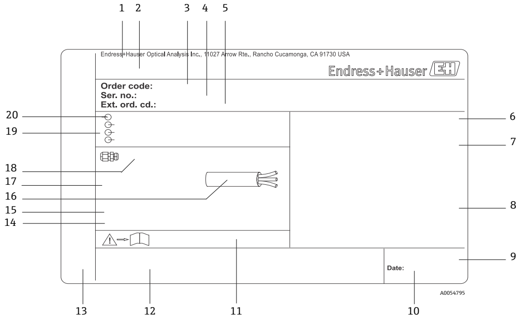
Figure 4. J22 TDLAS gas analyzer nameplate template
