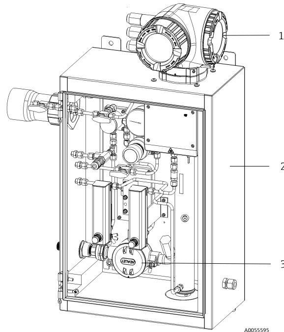
Figure 3. J22 TDLAS gas analyzer in an enclosure
