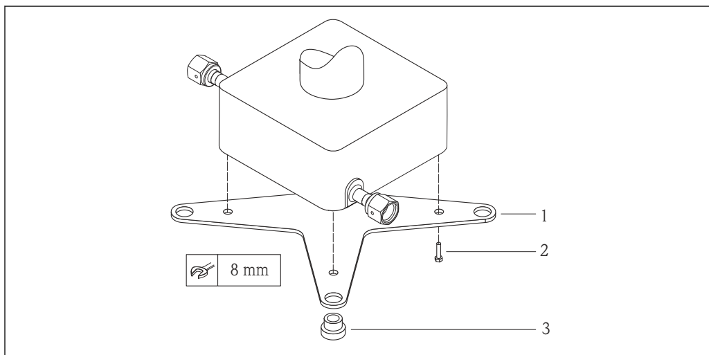
14 Mounting kit for Cubemass mounting plate
