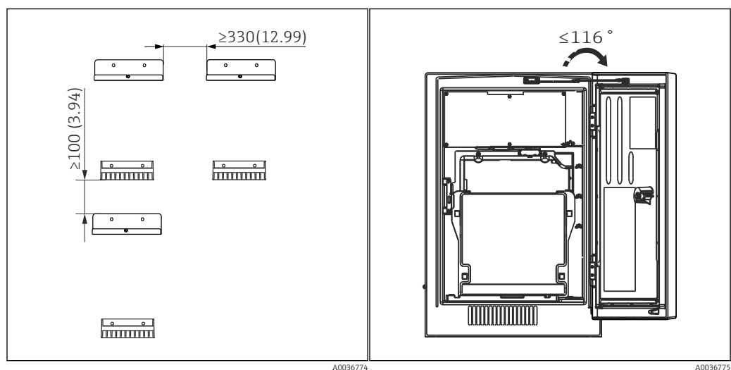
13 Minimum spacing required for installation. Unit of measurement mm (in) 14 Maximum opening angle
