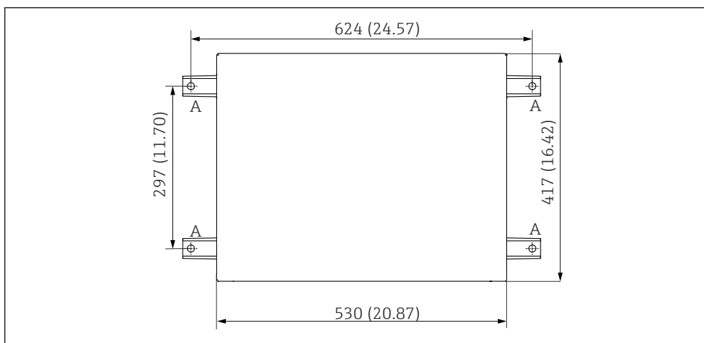
16 Foundation plan. Unit of measurement mm (in)
