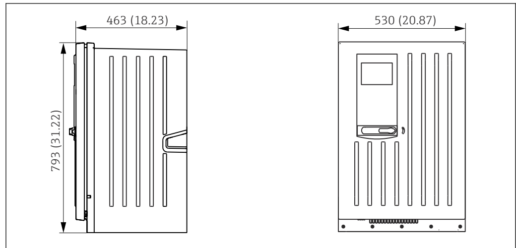
8 Enclosed installation. Unit of measurement mm (in)
