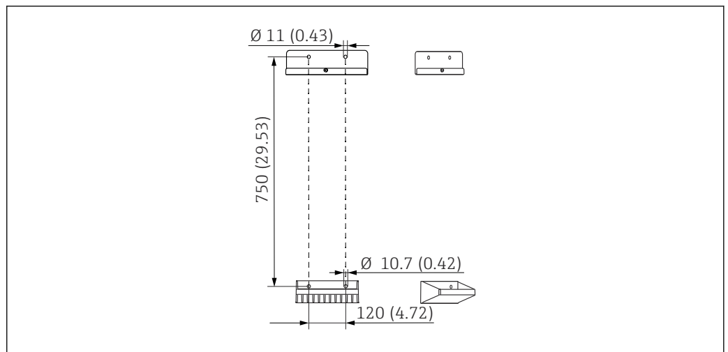
15 Dimensions of holder. Unit of measurement mm (in)
