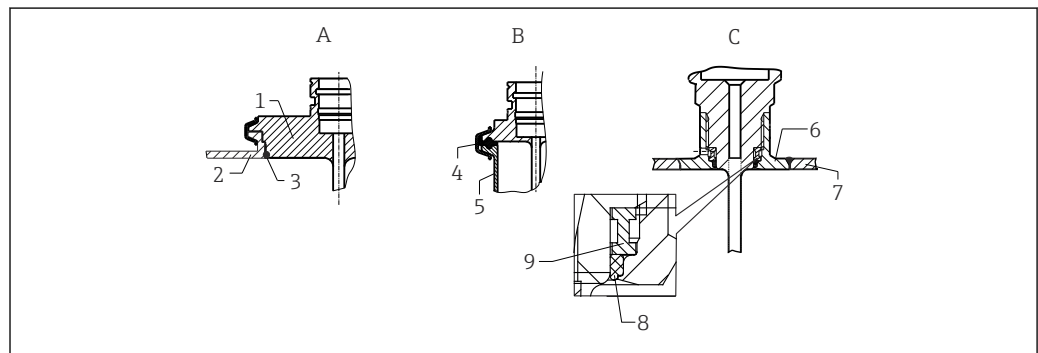
4 Detailed installation instructions for hygiene-compliant installation
