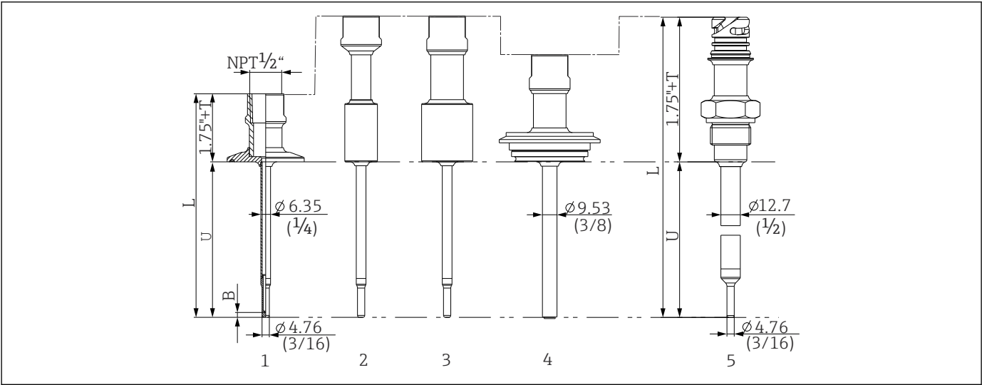
14 Thermowell with NPT 1/2" neck connection and various process connection versions:
