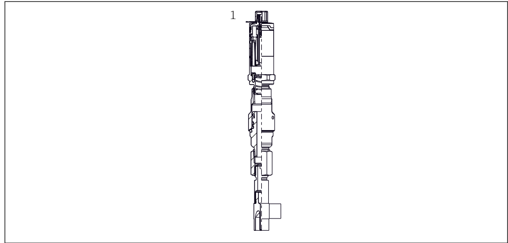
3 Process connections for thermometer installation in pipes with small nominal diameters
