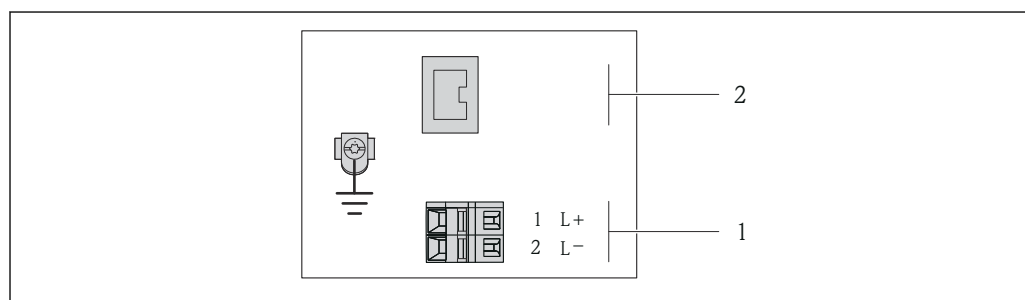
6 Occupation des bornes EtherNet/IP
