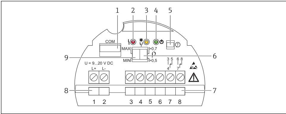
27 Example of electronic insert FEL64DC
