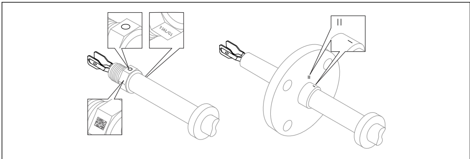
8 Position of the vibrating fork when installed horizontally in the vessel using the marking
