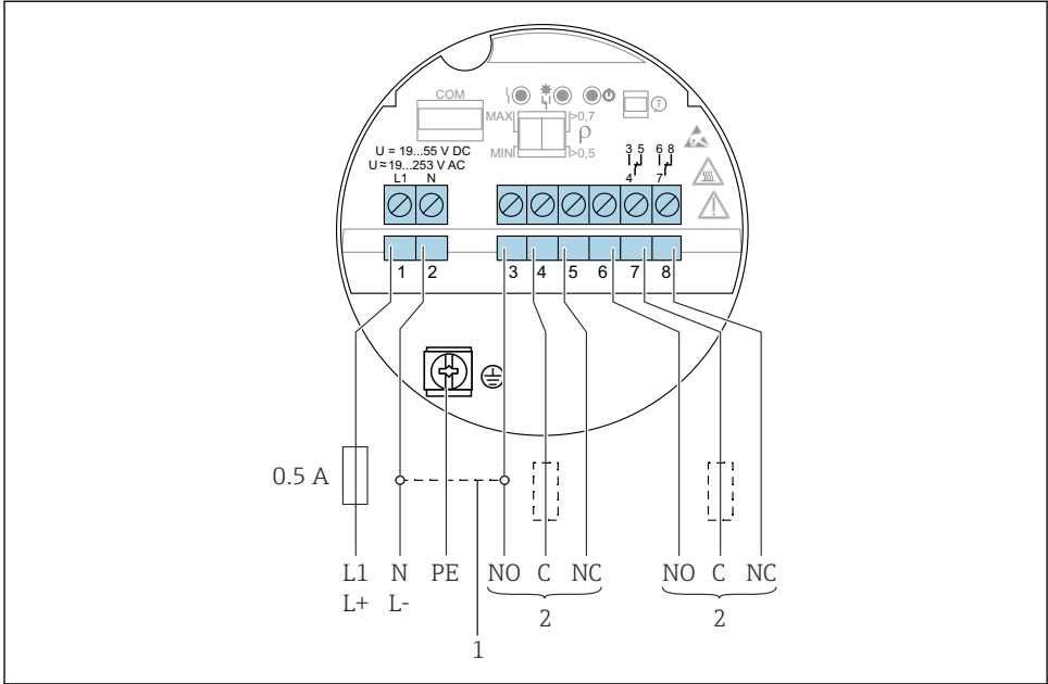
18 Universal current connection with relay output, electronic insert FEL64
