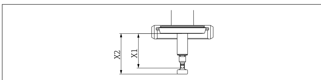
22 Immersion depth in mm (in) for process connection MA and MB thread
