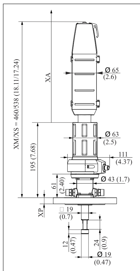
17 Manual drive, long version, dimensions in mm (in)
