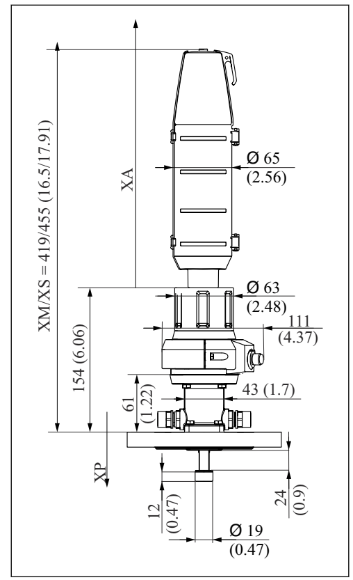
15 Manual drive, short version, dimensions in mm (in)
