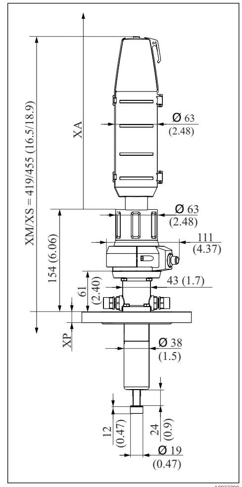
19 Immersion chamber version with manual drive, dimensions in mm (in)
