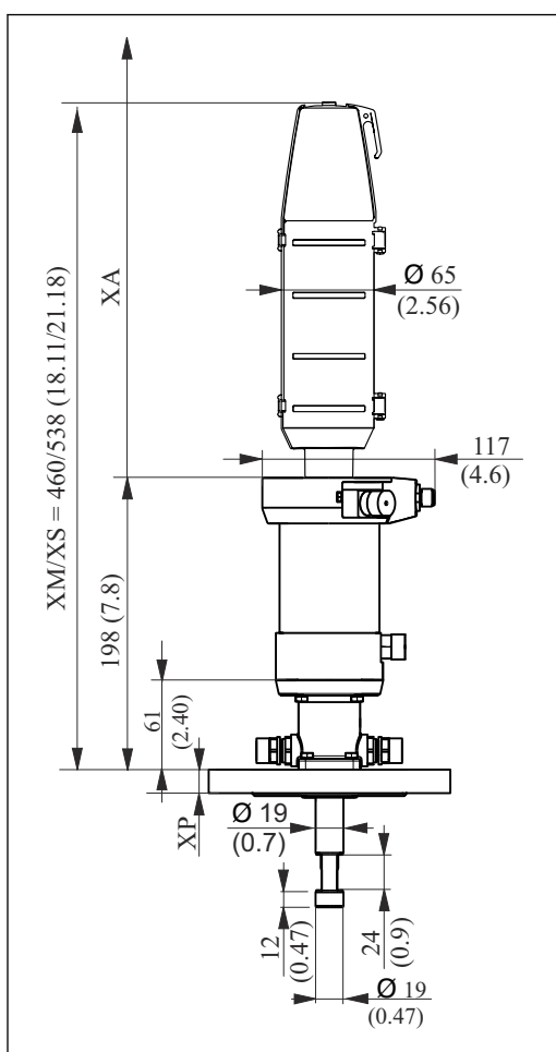
16 Pneumatic drive, long version, dimensions in mm (in)
