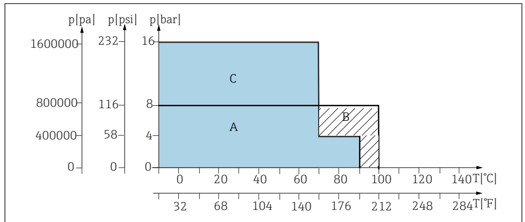
11 Pressure/temperature ratings for basic version for PVDF and conductive PVDF materials (CPA871-**G/H***** )
