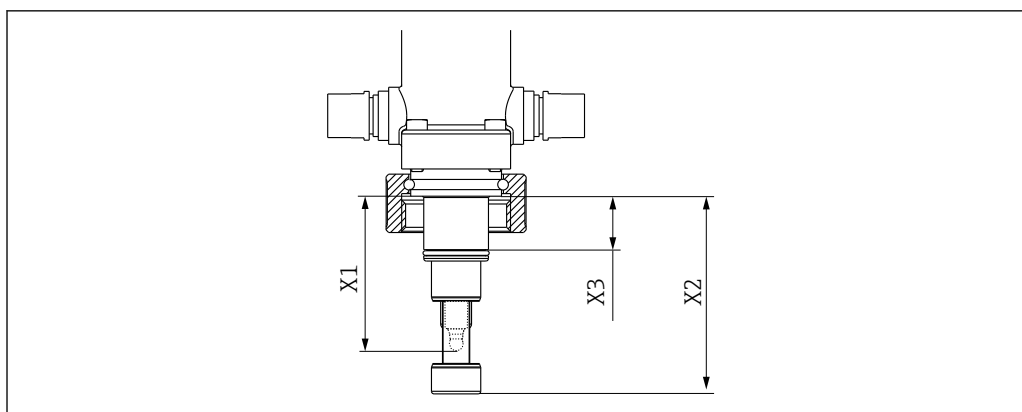
21 Immersion depth in mm (in) for process connection NA thread ISO 228 G1 1/4
