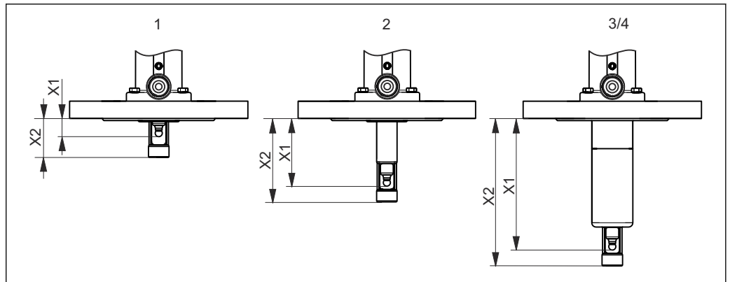
20 Immersion depths in mm (in)
