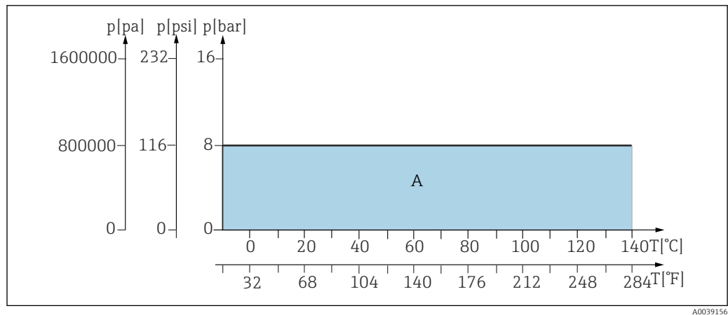
8 Pressure temperature ratings for basic and immersion chamber version for materials 1.4404, Alloy C22 and PEEK
