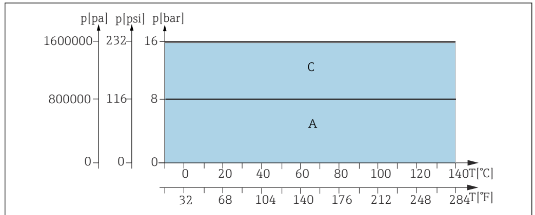
10 Pressure/temperature ratings for basic and immersion chamber version for 1.4404, Alloy C22 and PEEK materials (CPA871-**G/H***** )
