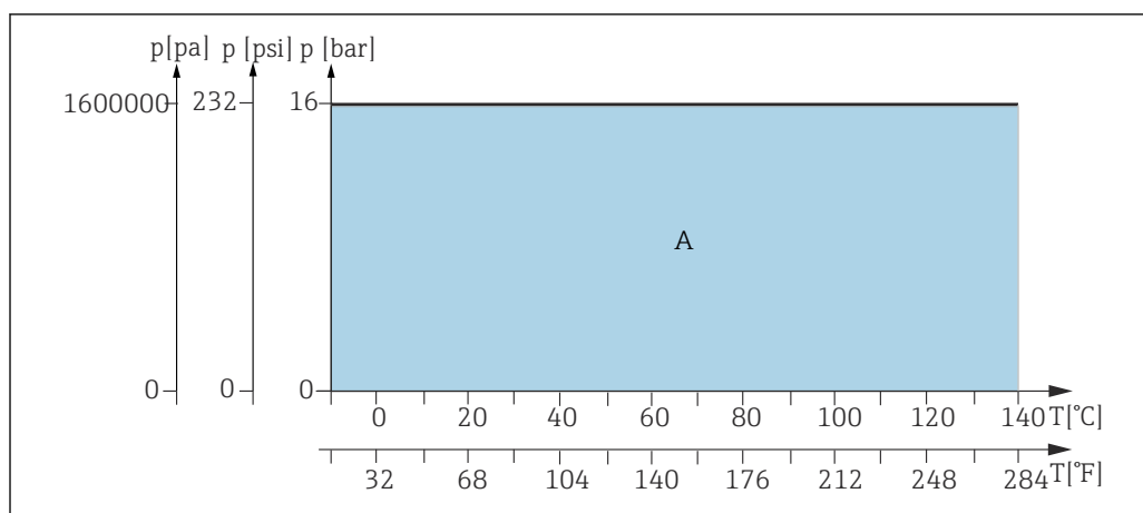
12 Pressure/temperature ratings for basic and immersion chamber version for 1.4404, Alloy C22 and PEEK materials (CPA871-**E/F*****)
