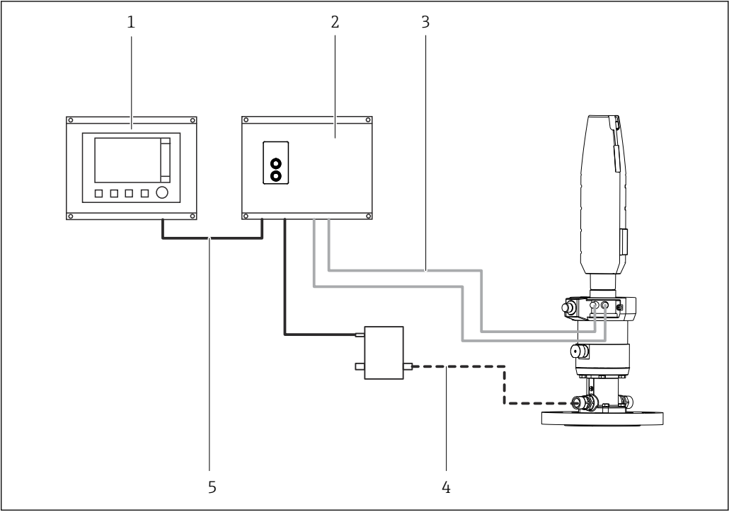
6 Cleaning control with Cleanfit Control
