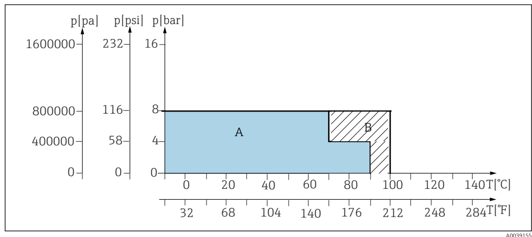
9 Pressure temperature ratings for basic version for materials PVDF and conductive PVDF
