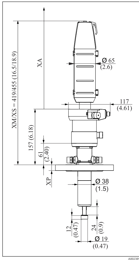
18 Immersion chamber version with pneumatic drive, dimensions in mm (in)
