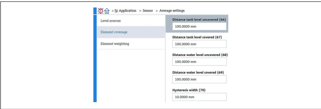
82 Element coverage 子菜单界面
