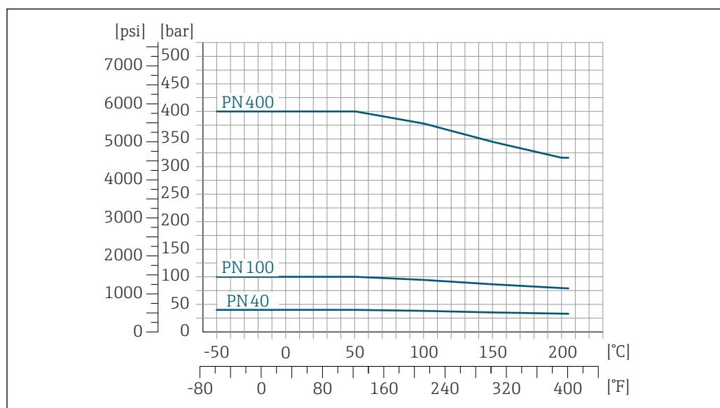
16 Com material do flange: 1.4404 (316/316L)
