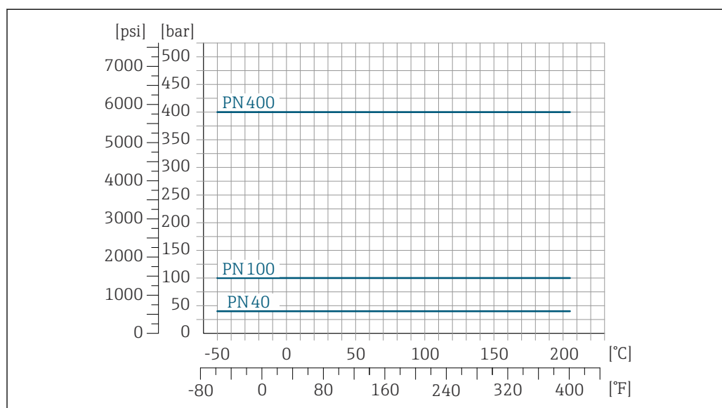
17 Com material do flange: Liga C22, 2.4602 (UNS N06022)
