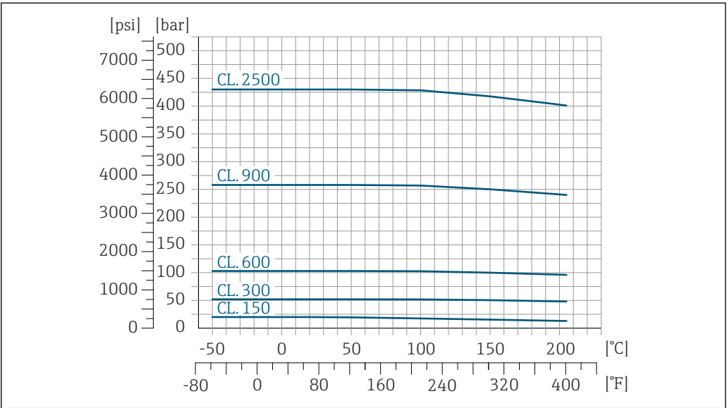
20 Com material do flange: Liga C22, 2.4602 (UNS N06022)
