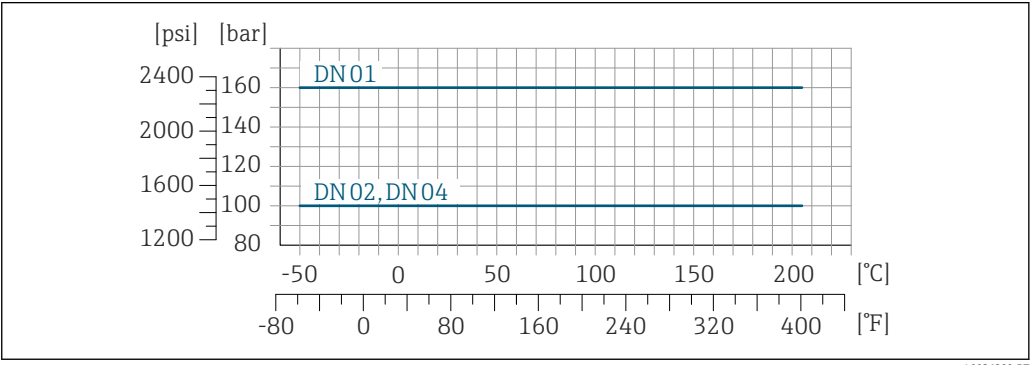
24 Com material do flange: 1.4404 (316/316L)
