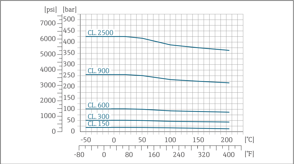
19 Com material do flange: 1.4404 (316/316L)
