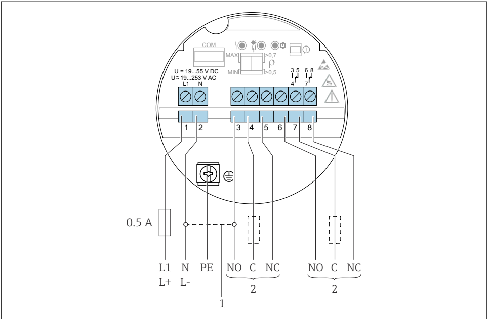
21 Universal current connection with relay output, electronic insert FEL64
