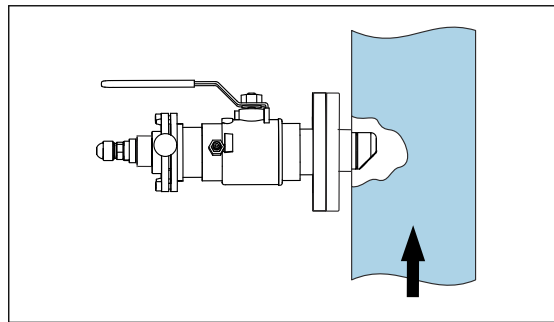
12 Installing with CUA451 retractable assembly
