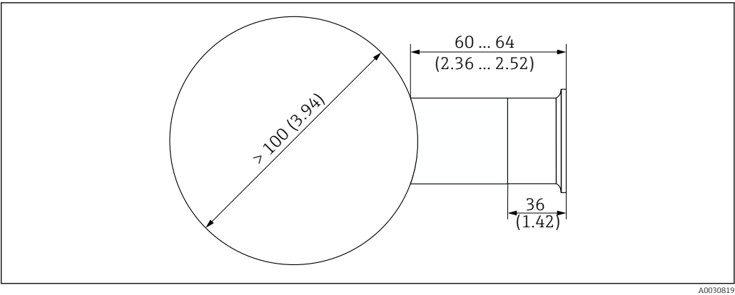
19 Pipe connection with weld-in adapter. Dimensions: mm (in)
