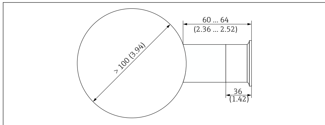
26 Pipe connection with weld-in adapter. Unit: mm (in)
