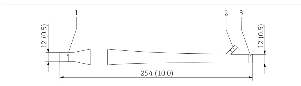
29 Bubble trap. Unit: mm (in)
