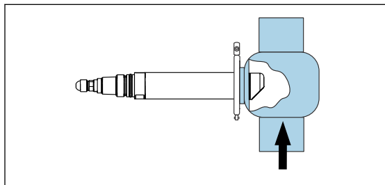
17 Installing with standard Varivent connection
