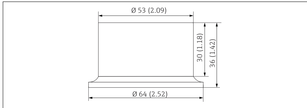
25 Weld-in adapter. Unit: mm (in)
