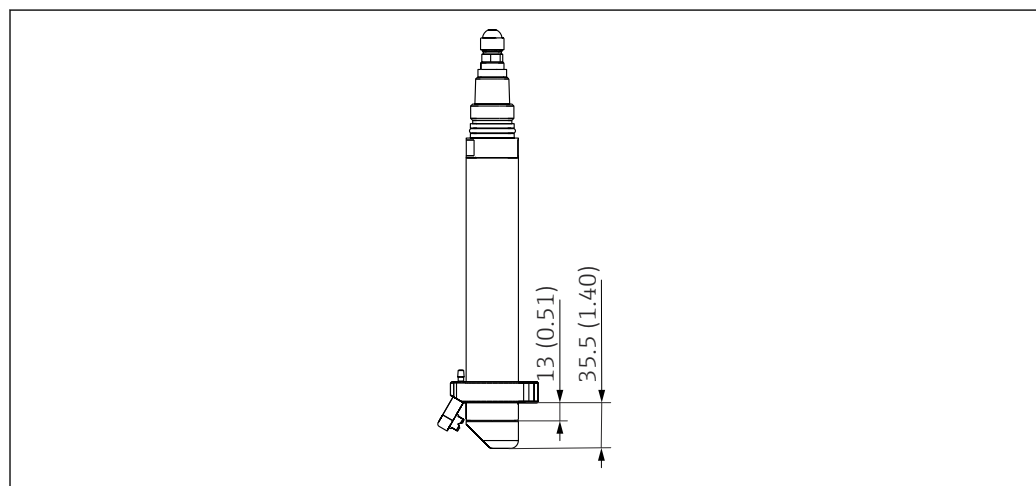
23 Dimensions of sensor with compressed air cleaning. Dimensions: mm (in)
