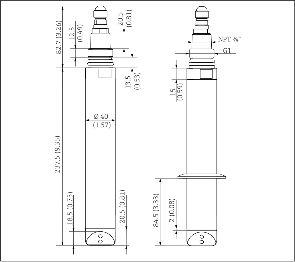
21 Dimensions of stainless steel sensor and stainless steel sensor with clamp connection (right). Dimensions: mm (in)
