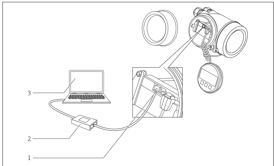
43 DeviceCare/FieldCare via interface service (CDI)
