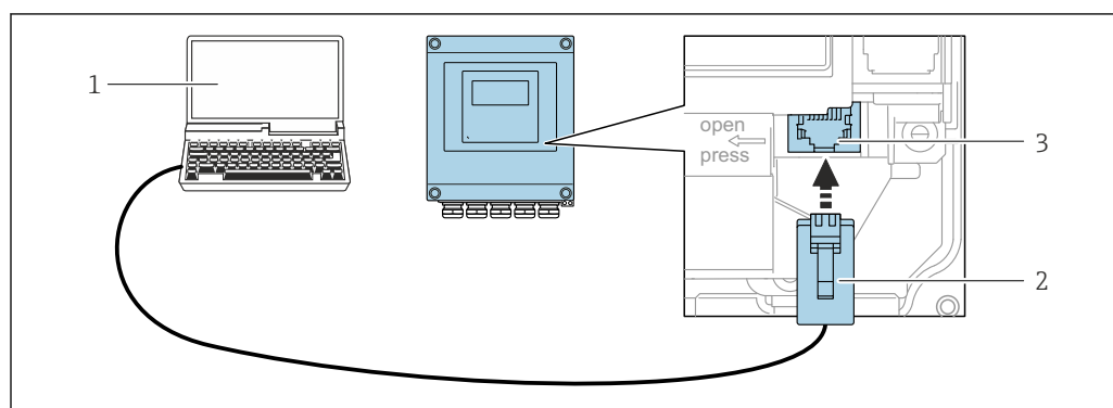
62 Raccordement via interface service (CDI-RJ45)
