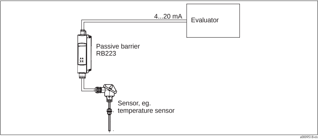
Fig. 2: Safety function with RB223
