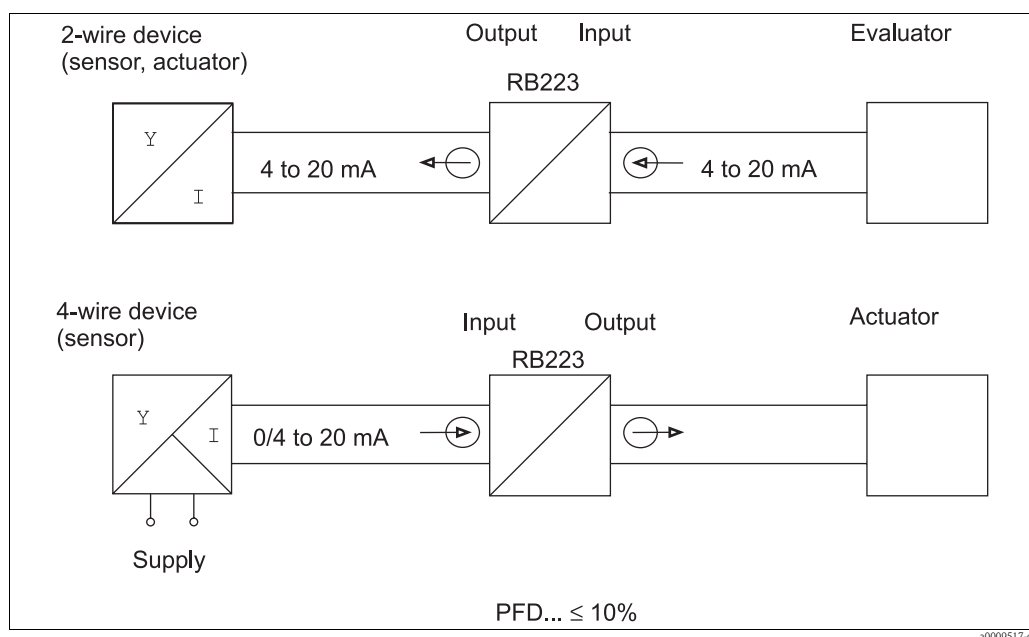
Fig. 1: Share of the passive barrier in the "average probability of dangerous failures of a safety function on demand" ( PFD_{AVG} )
