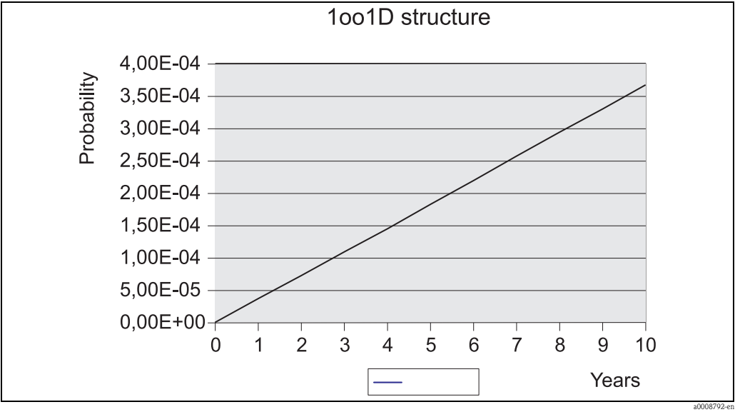
Figure: PDF_{av} against time interval for iterative tests (FMEDA report, Figure 3)
