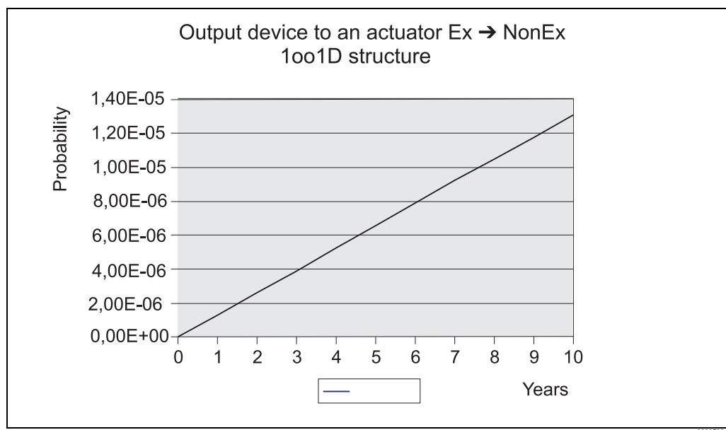
Figure: PFD_{av} against time interval for iterative tests (FMEDA report, Figure 4)
