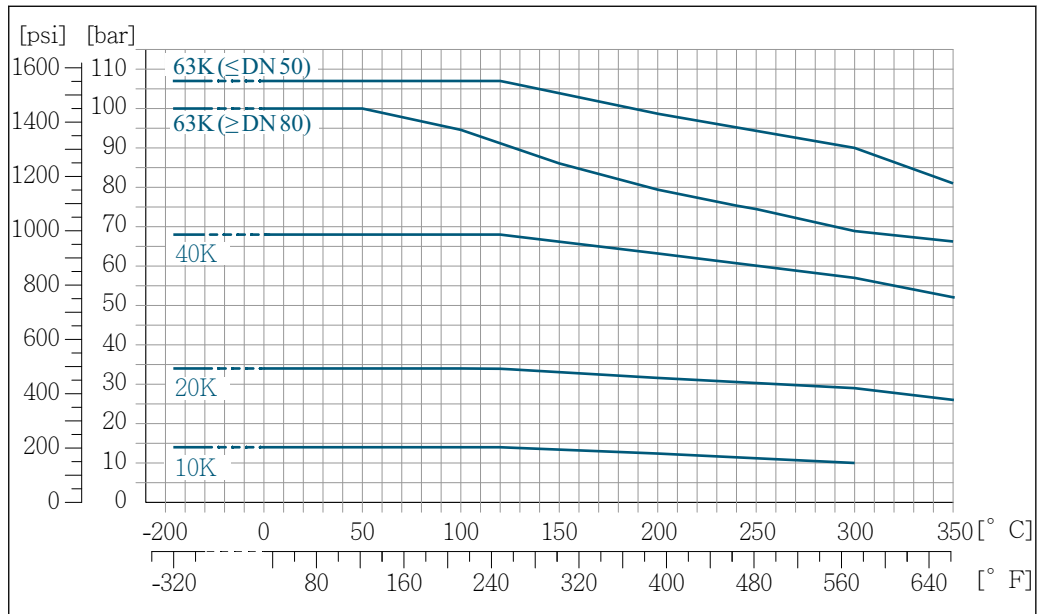
19 Com material do flange 1.4404 (F316/F316L), Liga C22
