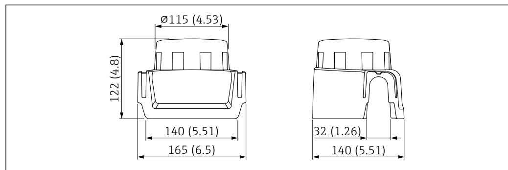
47 Protective cover for aluminum single compartment housing. Unit of measurement mm (in)
