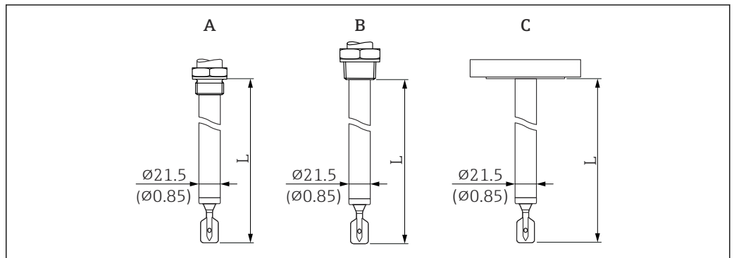
30 Probe designs: pipe extension, short pipe version (sensor length L). Unit of measurement mm (in)
