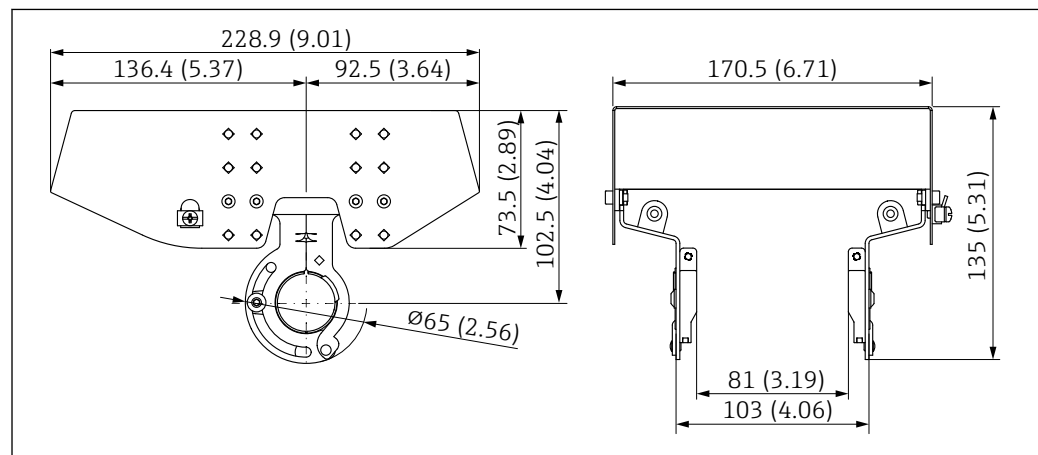
46 Weather protection cover for dual compartment housing. Unit of measurement mm (in)
