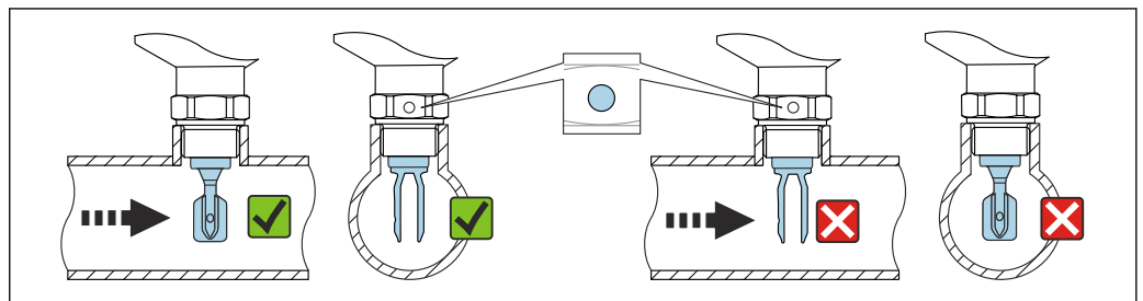
13 Installation in pipes (take fork position and marking into consideration)
