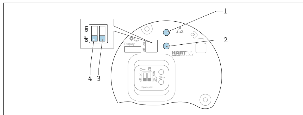
44 Operating keys and DIP switch on FEL60H electronic insert
