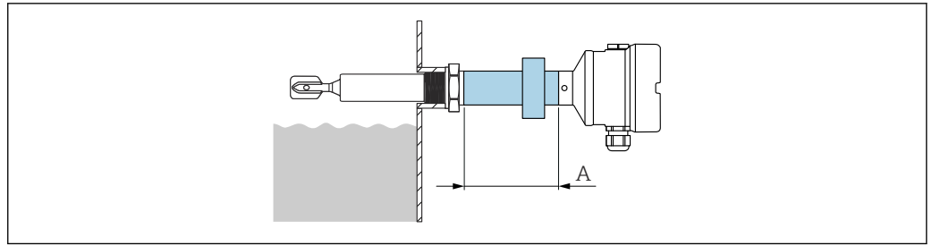
28 Ex d glass feedthrough for pipe extensions
