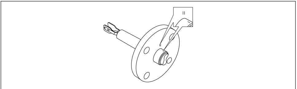
9 Position of the tuning fork when installed horizontally in the vessel using the marking
