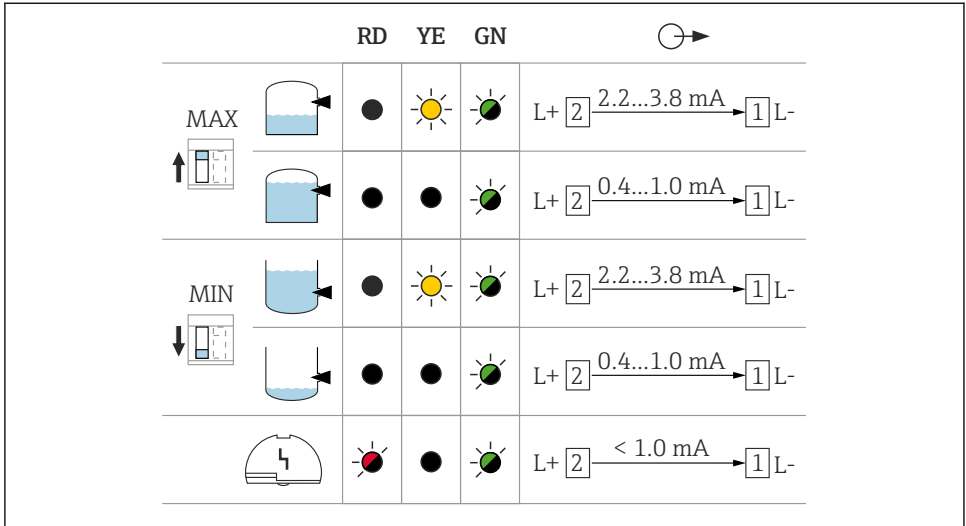
26 Behavior of switching output and signaling, electronic insert FEL68
