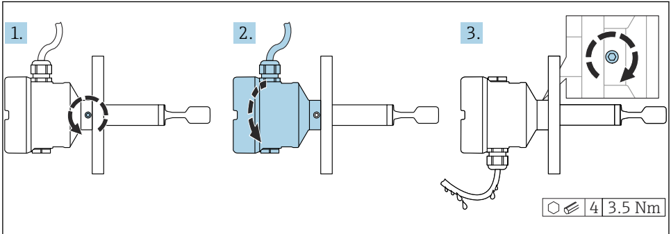
12 Housing with external locking screw; form a drip loop on the cable
