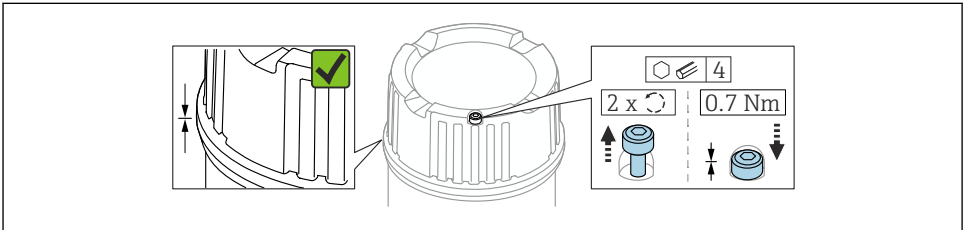
13 Cover with securing screw
