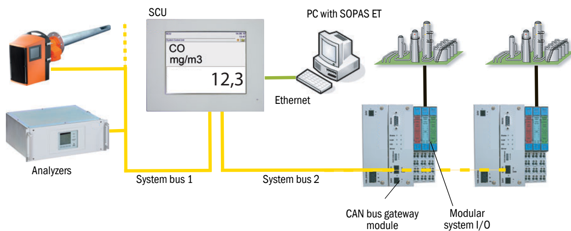
Fig. 4: Overview of subassemblies associated with the SCU
