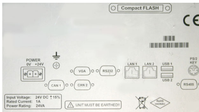
Fig. 6: Designation of connections on the back of the panel
