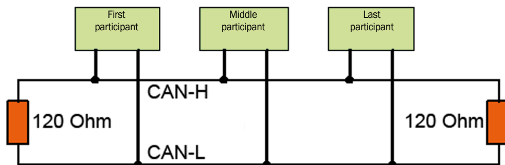
Fig. 8: CAN bus principle
