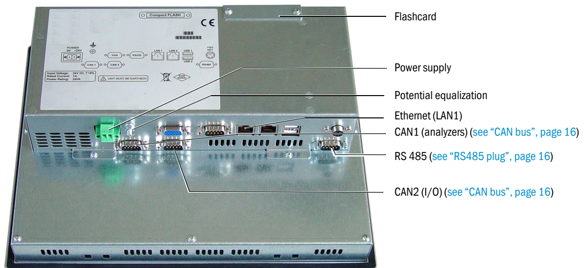
Fig. 5: Connections on the back of the panel
