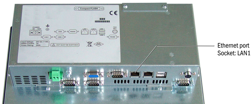
Fig. 11: Ethernet port on the back of the panel
