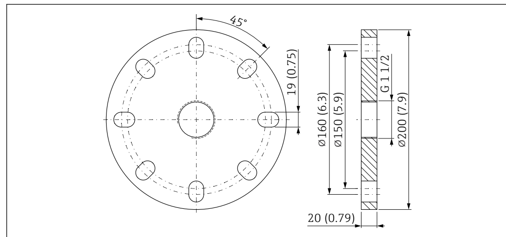
Brida UNI 3" / DN 80 / 80 A
