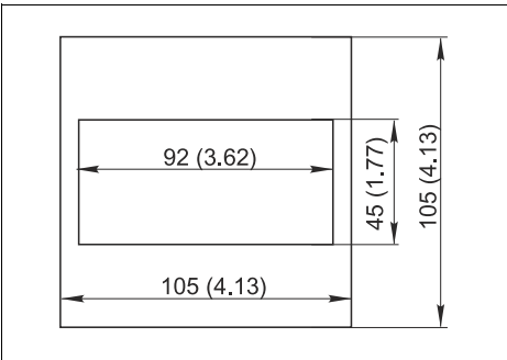
Fig. 4: Installed adapter frame in mm (inch)
