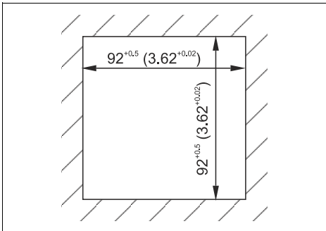
Fig. 3: Cabinet cutout in mm (inch)
