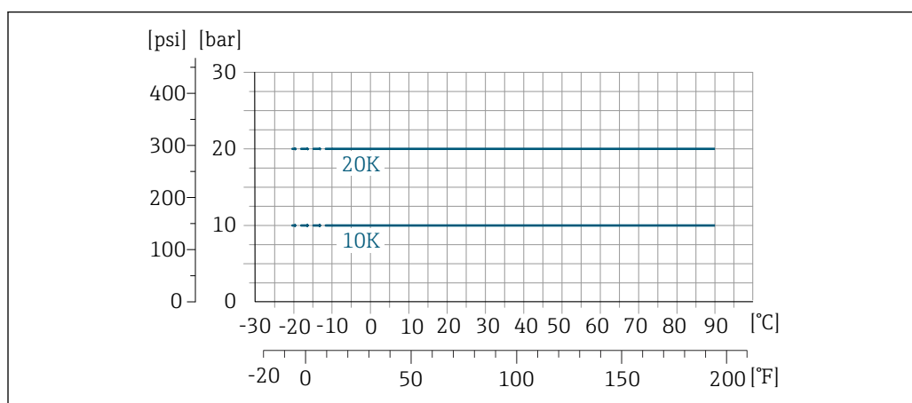
19 Matériau du raccord process : inox (-20 °C (-4 °F)) ; acier au carbone (-10 °C (14 °F))
