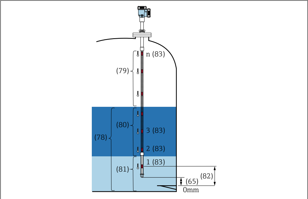
74 Element temperature
