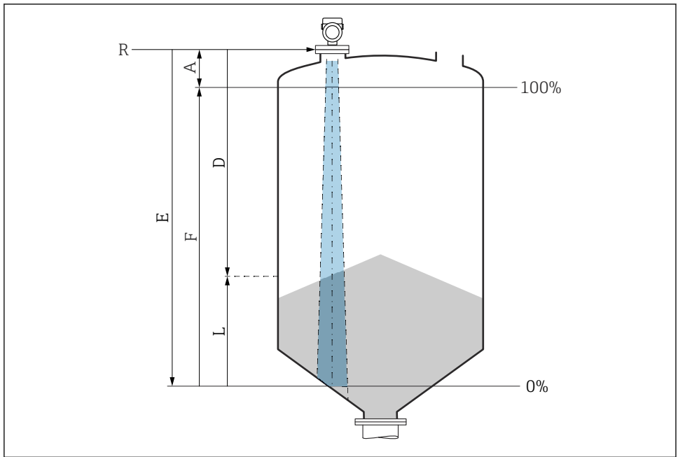
11 Configuration parameters for level measurement in bulk solids
