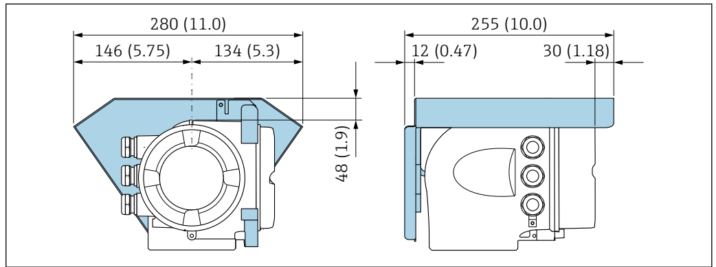
21 Weather protection cover for Proline 500 – unit mm (in)
