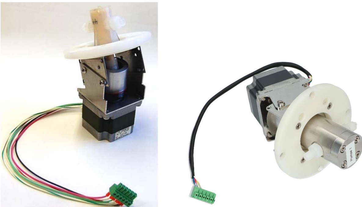
Figure 1: left: old pump 1000ul/stroke plastic head, 6 wires, right: new pump 800ul/stroke metal head, 4 wires
