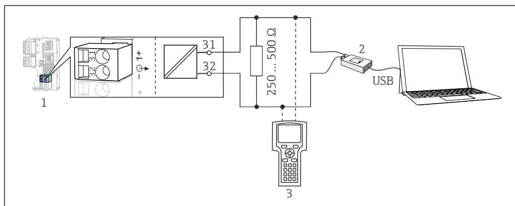
41 HART using modem
