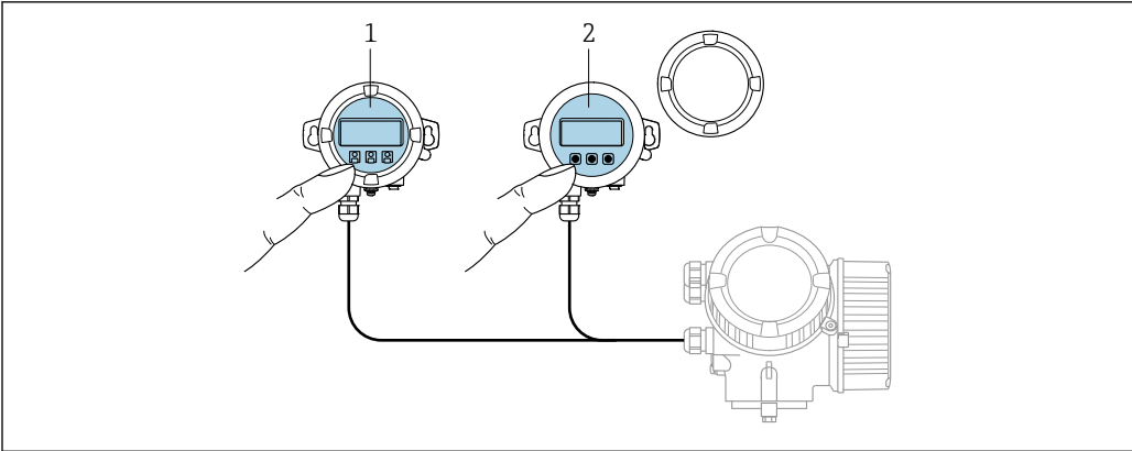
23 Options de configuration via FHX50
