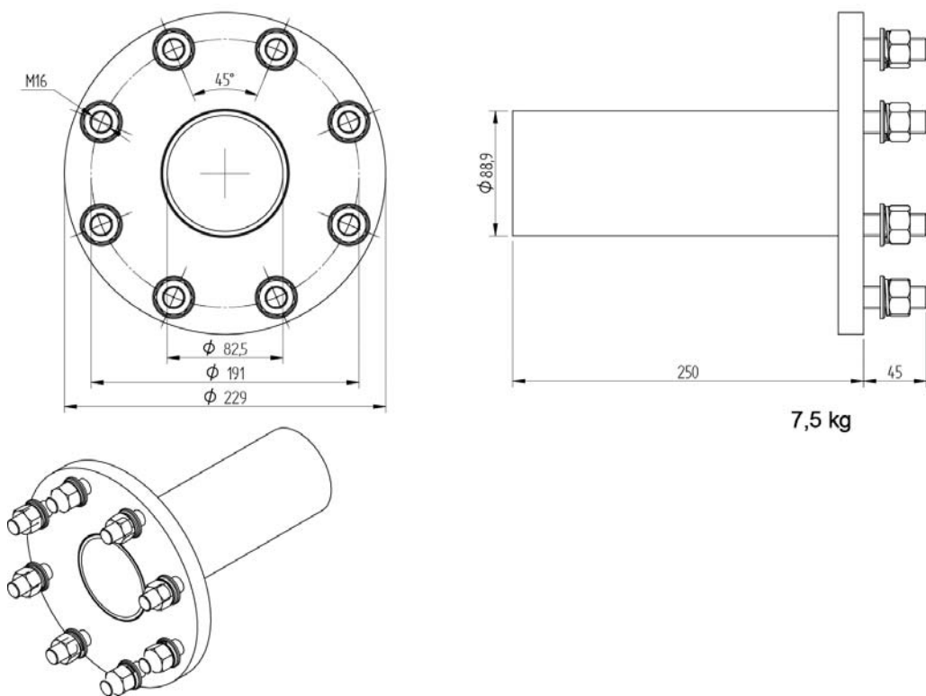
Fig. 15: Dimensions of counterflange with tube (others on request)
