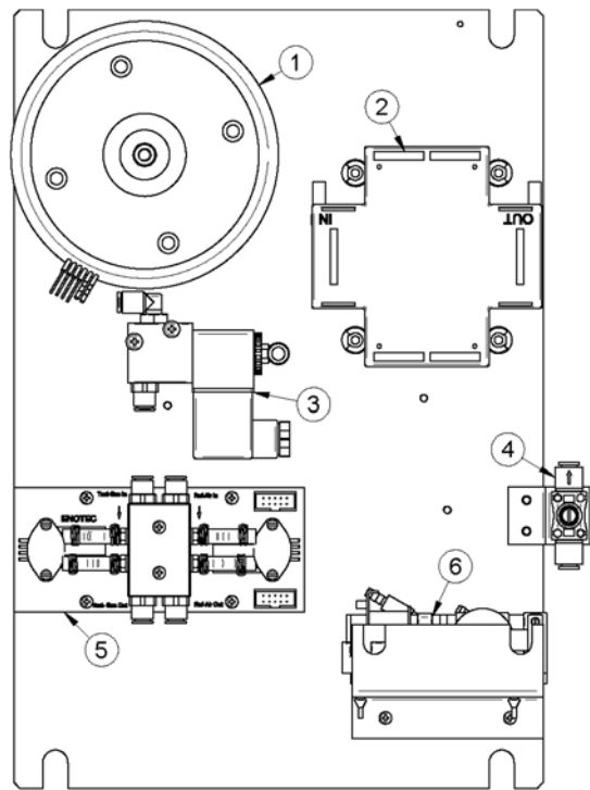
Field enclosure pump version Installation plate 1
