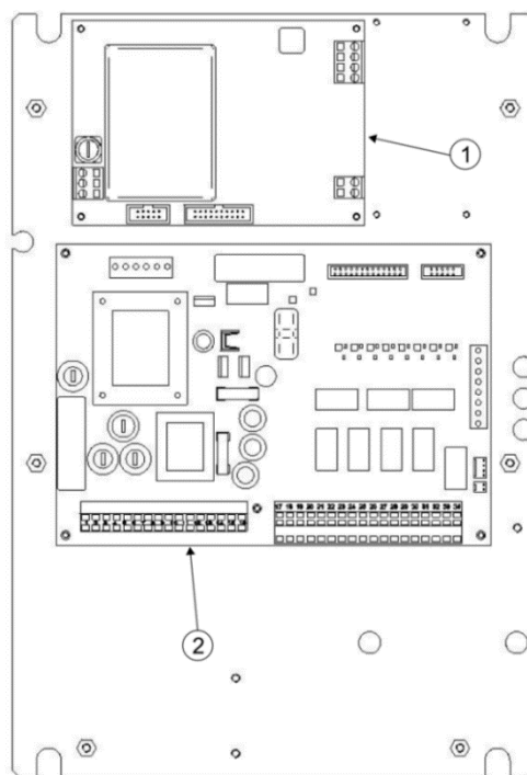
Field enclosure instrument air version installation plate 2
