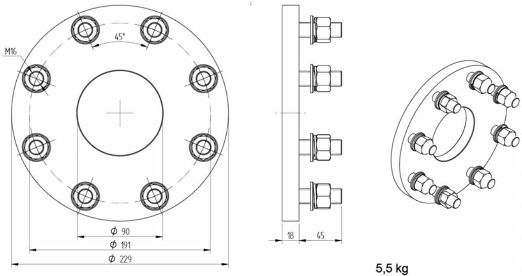
Fig 14: Counterflange dimensions
