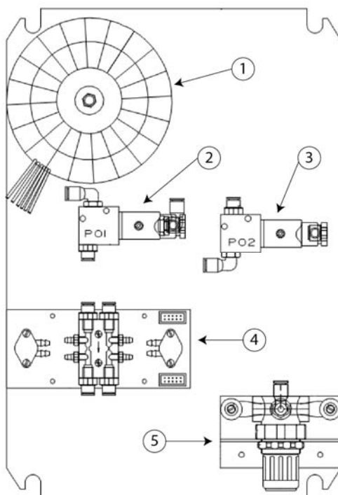
Field enclosure instrument air version installation plate 1
