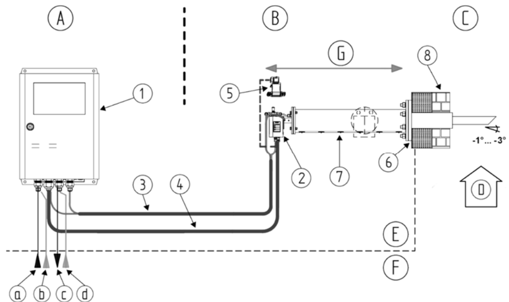
Fig 3: ZIRKOR200 with cooling protection tube for flue gas temperatures up to 1,600 °C
