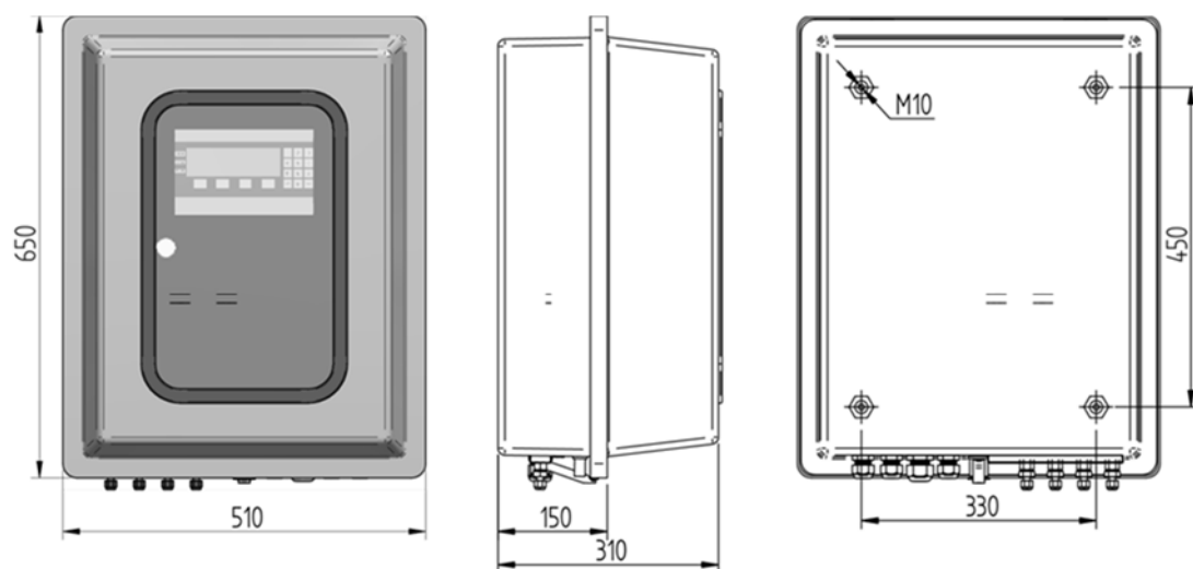
Fig 13: GRP protective box (option) – dimensions in mm
